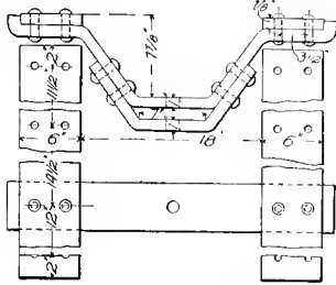
Figs. 1370-1371. Lever Fulcrum.
